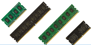
▶ Memory Upgrades
